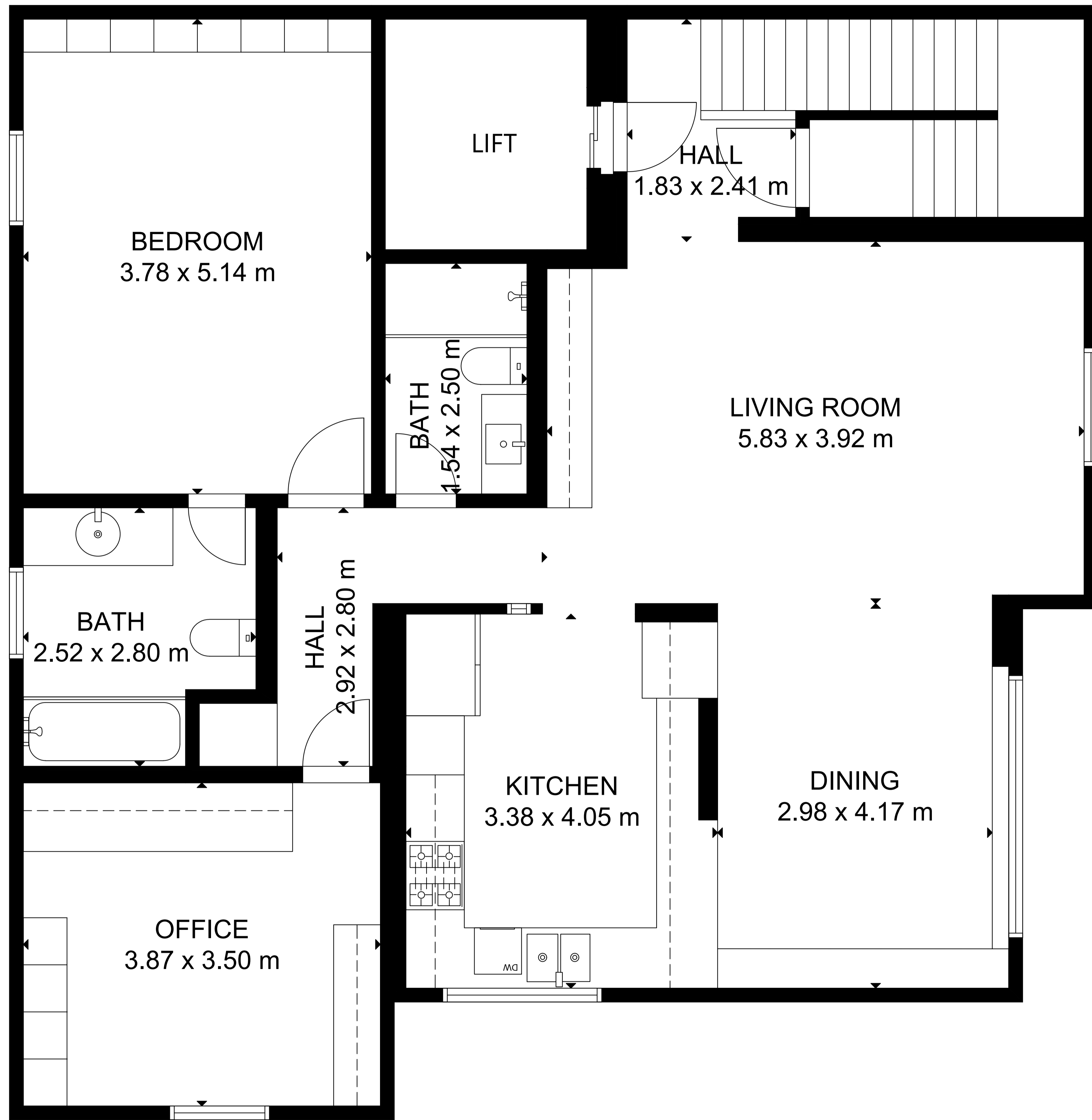
FLOOR 1
